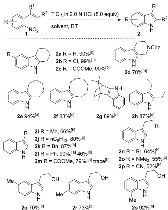
Scheme 2. General conditions: 1 (0.2 mmol), \text{TiCl}_3 (20% solution in 2.0 N HCl, 1.6 mmol), solvent ( c = 0.2 \text{ M} ), RT, 8 h. [a] Acetone as co-solvent. [b] Acetonitrile as co-solvent ( c = 0.4 \text{ M} ).
