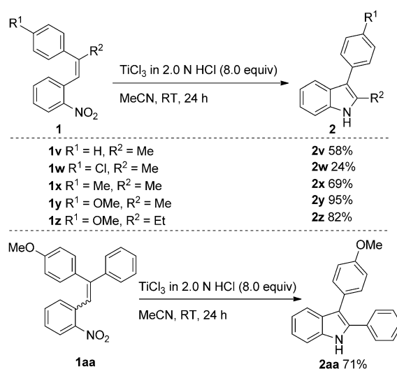
Scheme 4. Domino process involving N -cyclization and aryl migration.
