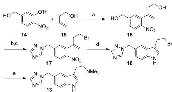
Scheme 7. Synthesis of rizatriptan. [a] Pd_2(dba)_3 (0.05 equiv), dppf (0.12 equiv), urotropine (2.0 equiv), THF, 80°C, 48 h, 91%. [b] CBr_4 , PPh_3 , CH_2Cl_2 , 0°C, 2 h, 83%. [c] Sodium salt of 1 H -1,2,4-triazole, DMF, –20°C, 2 h, 64%. [d] TiCl_3 (8.0 equiv), MeCN, RT, 4 h, 51%. [e] Dime-thylamine (excess), MeOH, 50°C, 48 h, 98%. dba = dibenzylidenace-tone, dppf = 1,1'-bis(diphenylphosphanyl)ferrocene, THF = tetrahydro-furan, and DMF = N,N -dimethylformamide.
